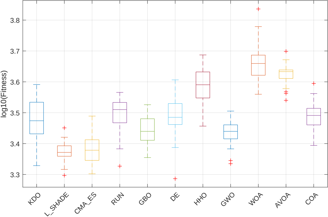
CEC2017 F17 (Numerical) - Boxplot
